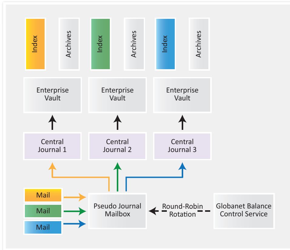
Figure 2: Globanet Balance Journal Infrastructure
