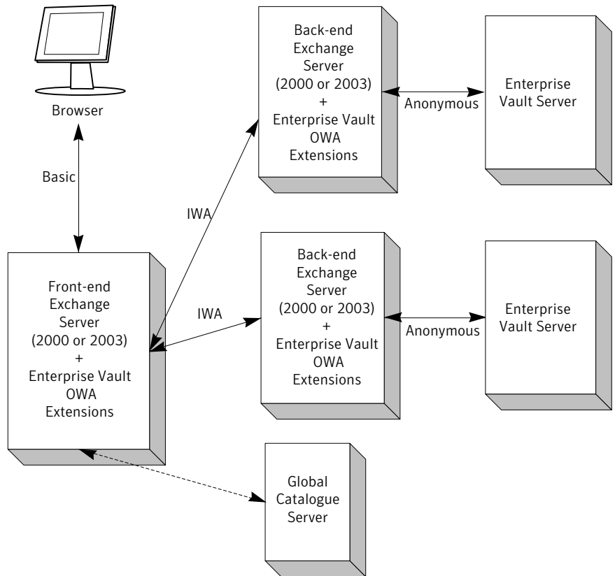
Figure 9-4 Front-end/back-end Exchange Server 2000 or 2003 OWA configuration
