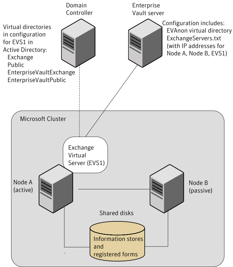
Figure 11-5 Detail of OWA 2003 and OWA 2000 Extensions configuration
