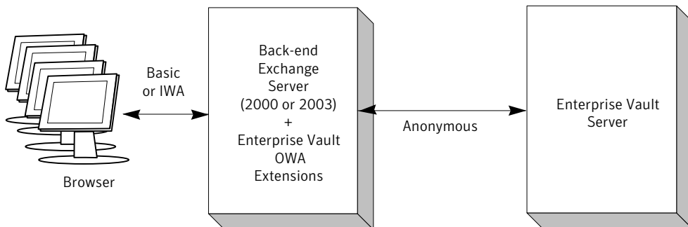
Figure 9-5 Back-end only Exchange Server 2000 or 2003 OWA configuration
