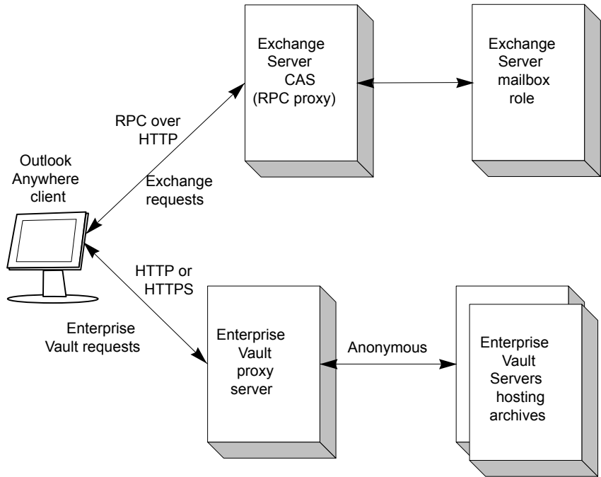
Figure 10-3 Example Outlook Anywhere configuration using an Enterprise Vault proxy server
