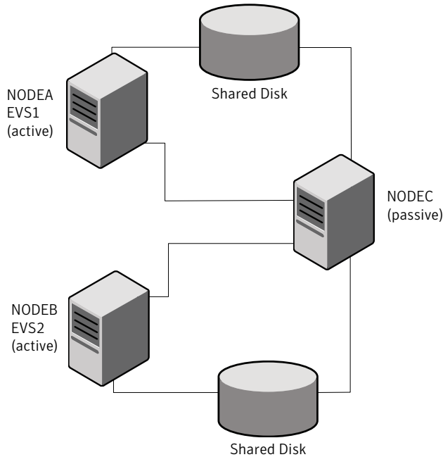
Figure 11-2 N+1 configuration
