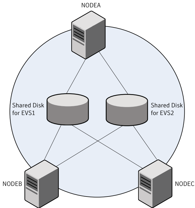
Figure 11-3 Alternative N+1 configuration
