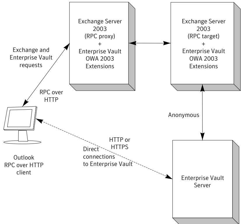
Figure 10-1 Example Outlook RPC over HTTP client and Exchange Server 2003 configuration
