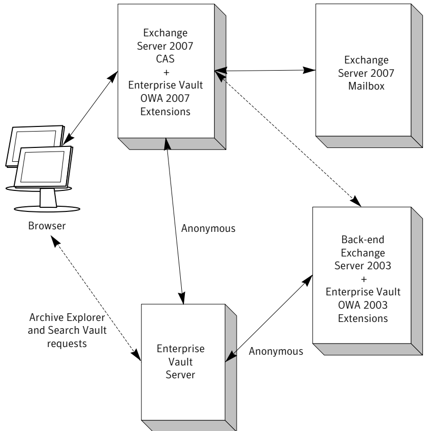
Figure 9-3 Mixed Exchange Server 2007 and 2003 OWA configuration
